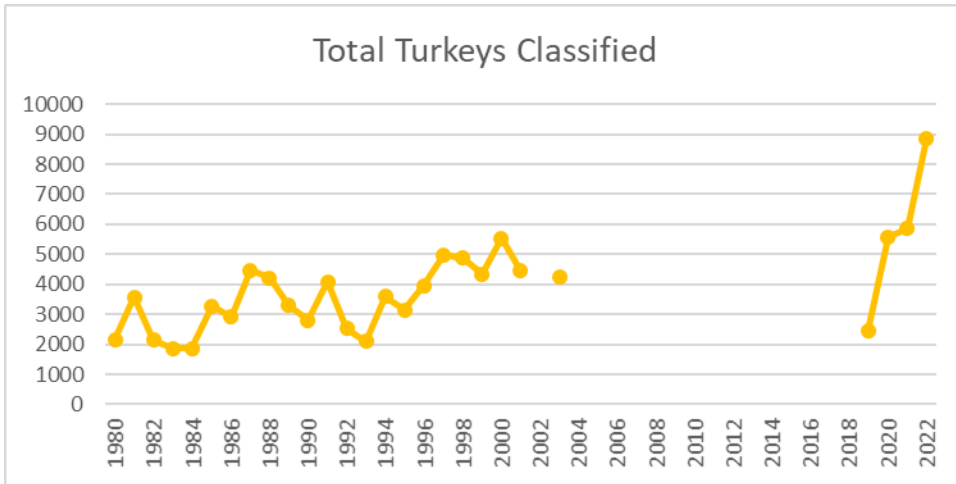
Figure 3. Total Turkeys Classified.
