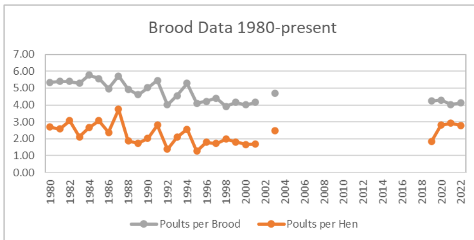
Figure 1. Historic Average Brood Size and Poults per Hen.
