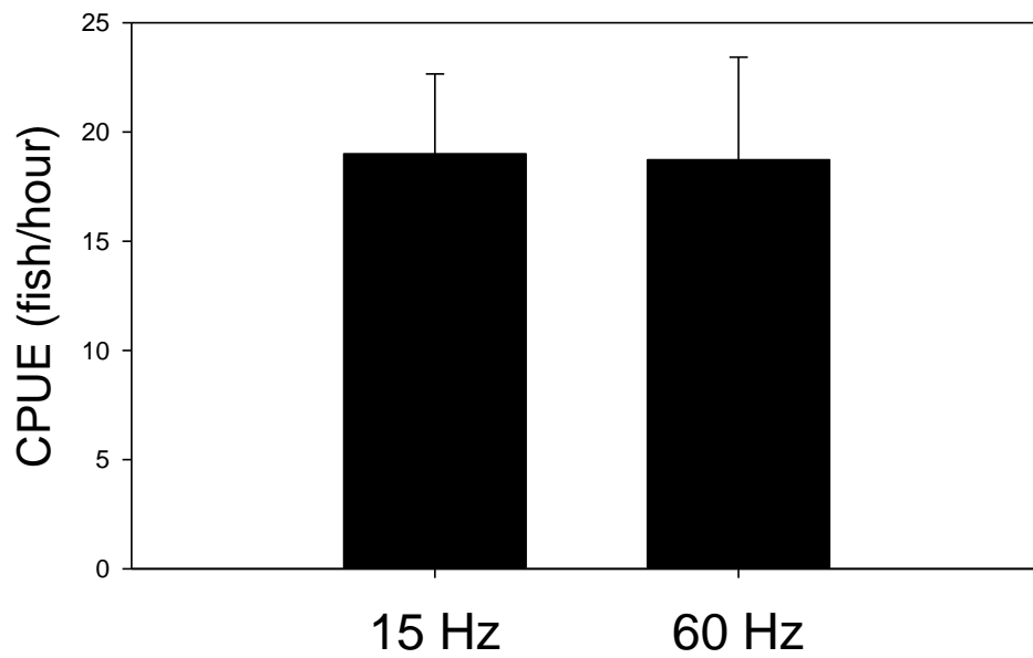
Figure 3. Standard sampling channel catfish mean catch per unit effort (CPUE) of 25-mm (4-hoop) hoop nets, electrofisher (15 Hz), and electrofisher (60 Hz) deployed in the Platte River, Nebraska during 2010.
