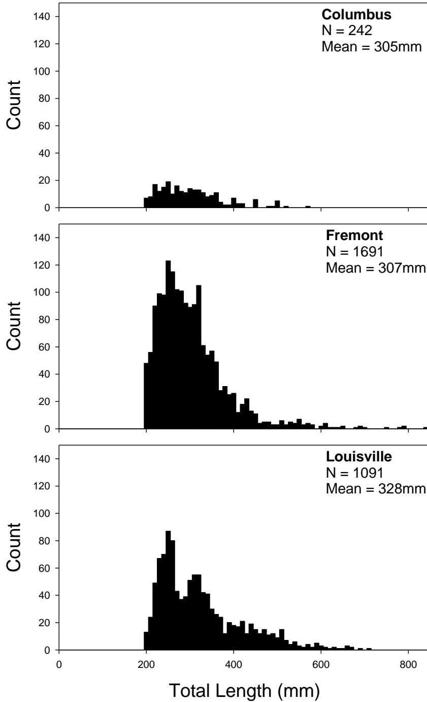
Figure 6. Tagging length-frequency distribution of channel catfish captured at Columbus, Fremont, and Louisville in the Platte River, Nebraska during 2010.
