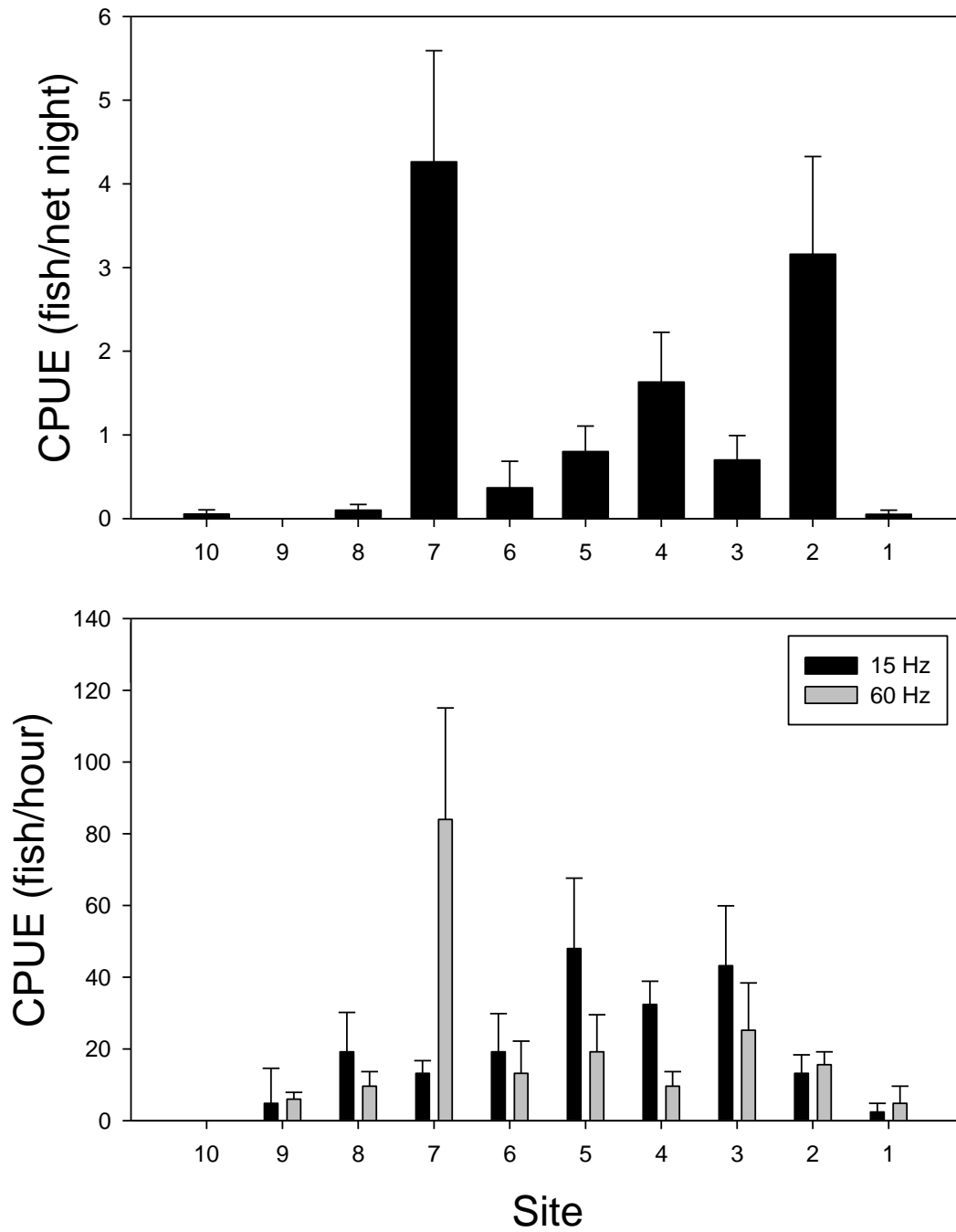
Figure 4. Standard sampling longitudinal channel catfish mean catch per unit effort (CPUE) of 25-mm (4-hoop) hoop nets, electrofisher (15Hz), and electrofisher (60 Hz) in the Platte River, NE during 2010.
