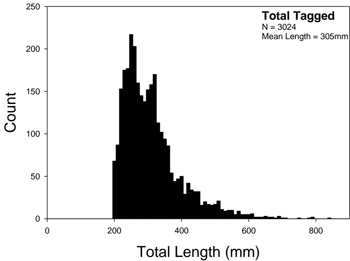
Figure 5. Tagging length-frequency distribution of channel catfish caught in all gears in the Platte River, Nebraska during 2010.
