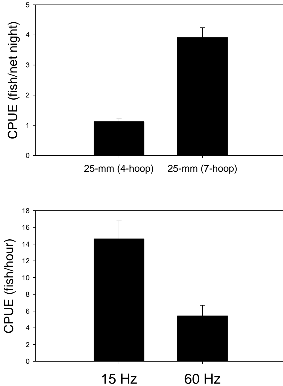
Figure 7. Tagging mean catch per unit effort (CPUE) of channel catfish greater than 200-mm captured by 25-mm (4-hoop) hoop net, 25-mm (7-hoop) hoop net, electrofisher (15Hz), and electrofisher (60Hz) in the Platte River, Nebraska during 2010.
