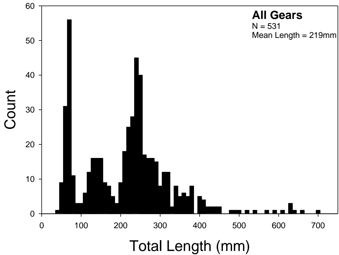
Figure 1. Standard sampling length-frequency distribution of channel catfish caught in all gears in the Platte River, Nebraska during 2010.
