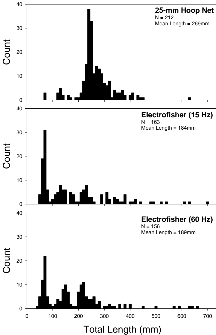
Figure 2. Standard sampling length-frequency distribution of channel catfish captured by 25-mm hoop net, electrofisher (15Hz), and electrofisher (60Hz) in the Platte River, Nebraska during 2010.
