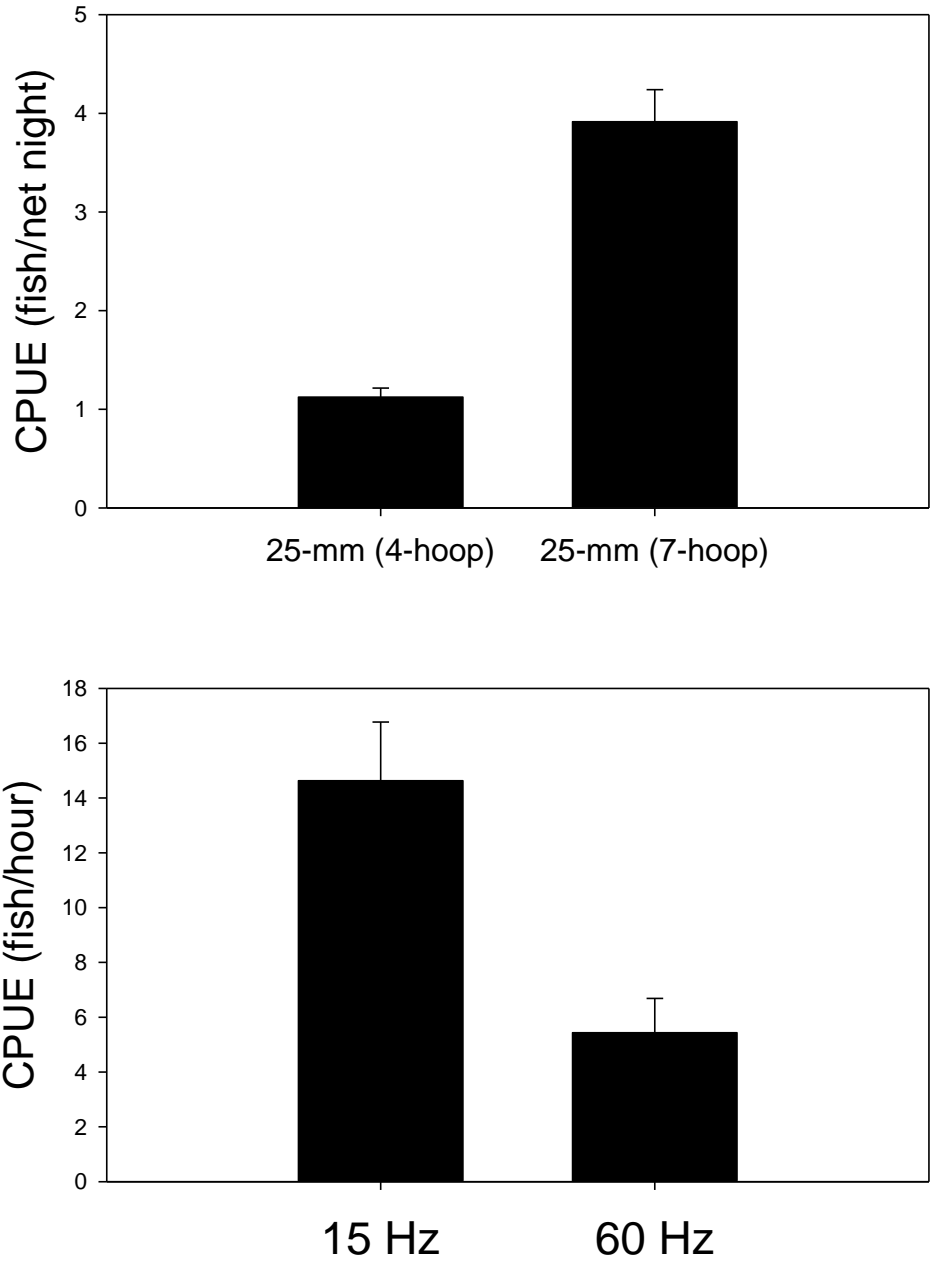
Figure 9. Tagging mean catch per unit effort (CPUE) of flathead catfish greater than 200-mm captured by 25-mm (4-hoop) hoop net, 25-mm (7-hoop) hoop net, electrofisher (15Hz), and electrofisher (60Hz) in the Platte River, Nebraska during 2010.
