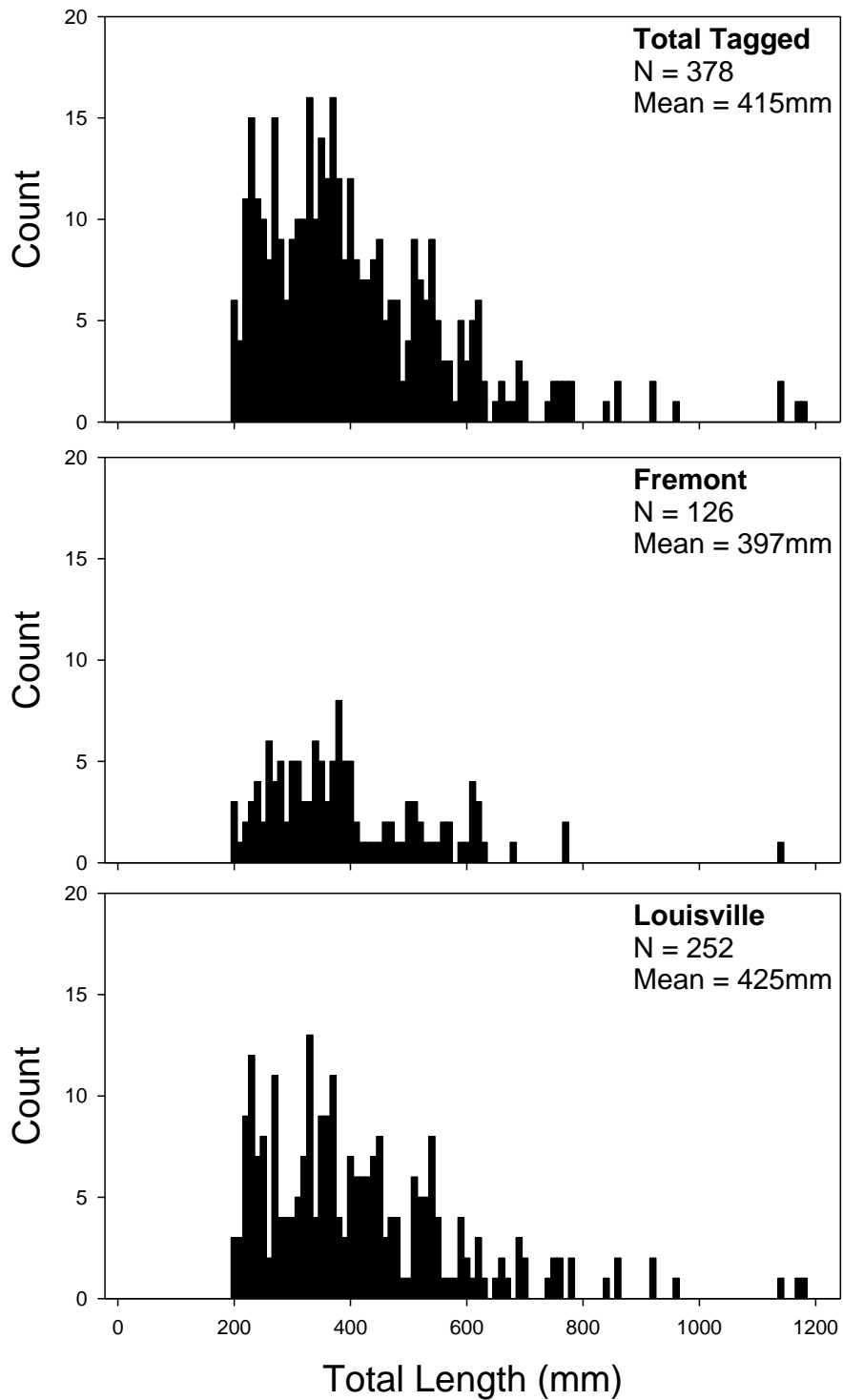
Figure 8. Tagging length-frequency distribution of flathead catfish captured by all gears, captured at Fremont, and captured at Louisville in the Platte River, Nebraska during 2010.
